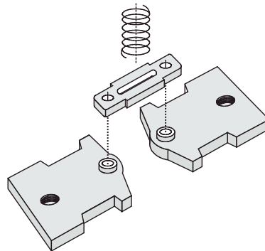
Contact Assembly
